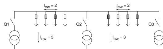
Triple infeed
