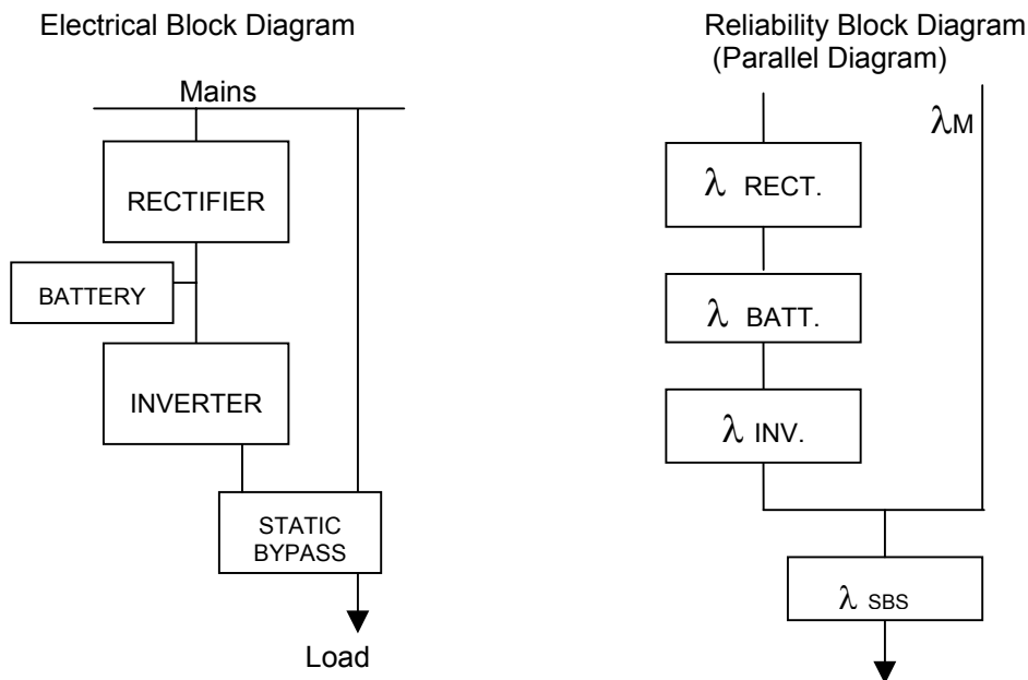
Fig. 2 Single UPS WITH static bypass. Electrical block diagram and reliability diagram
