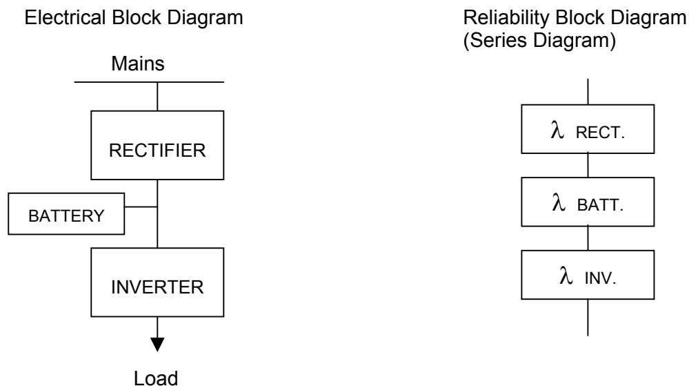
Fig. 1 Single UPS without static bypass. Electrical block diagram and reliability diagram
