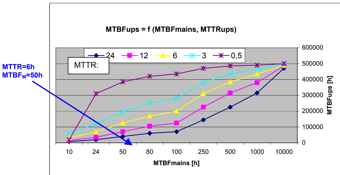
Fig. 3 This graph shows the dependence of the MTBF UPS+SBS on MTBF MAINS and MTTR UPS .
