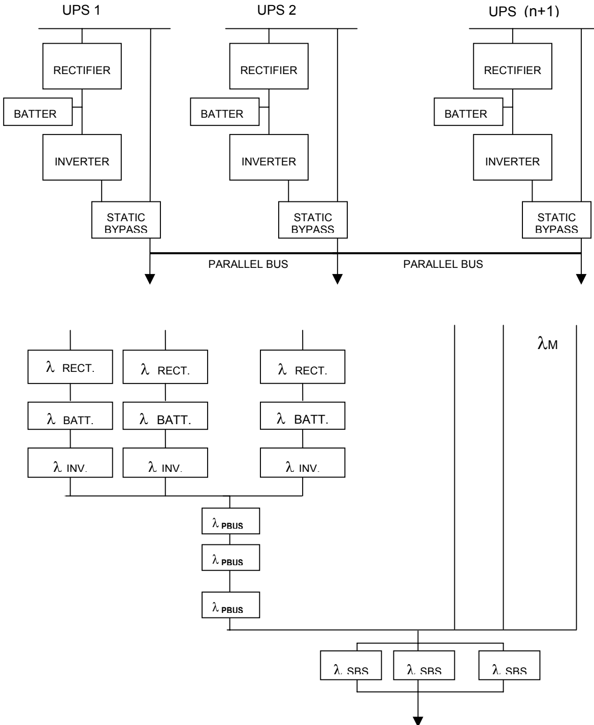
Fig. 4 Electrical and Reliability Block Diagram of (n+1) Parallel Redundant UPS Configuration.
