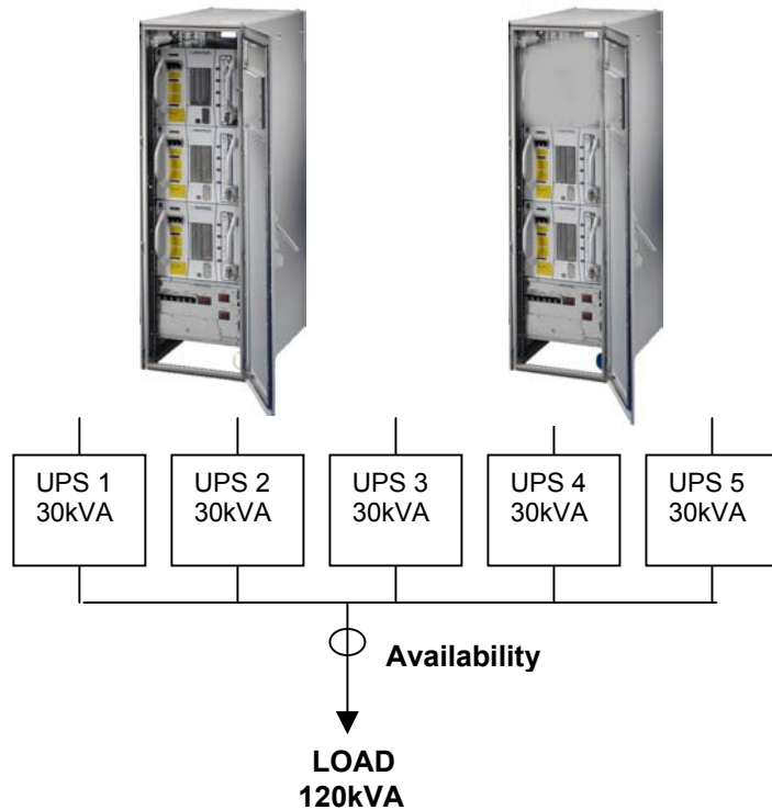
Fig. 5 Block diagram of two redundant UPS configurations
