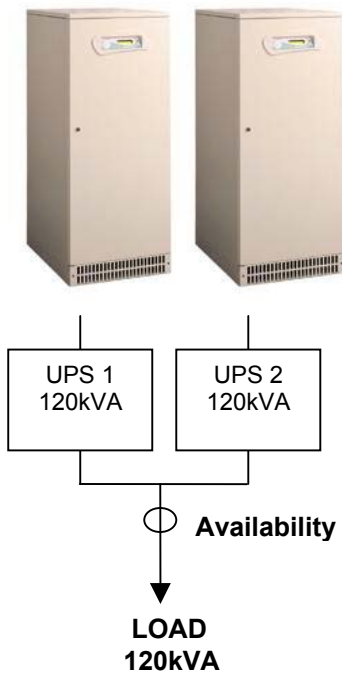
Fig. 5 Block diagram of two redundant UPS configurations
