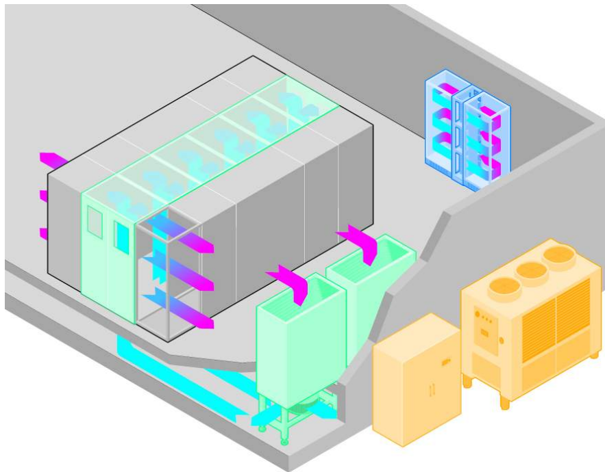
Figure 2: Aisle containment and CRAC system
