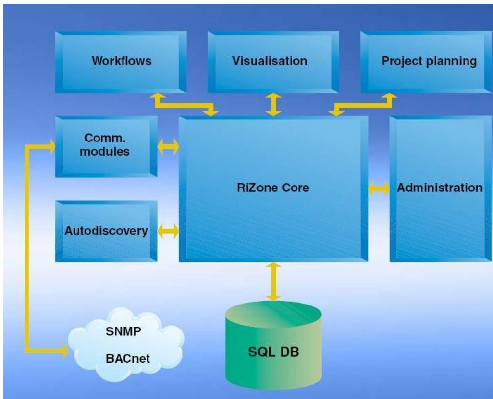
Figure 4: The RiZone architecture
