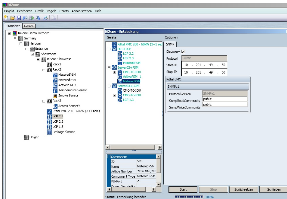
Figure 5: Autodiscovery for RiMatrix5 components
