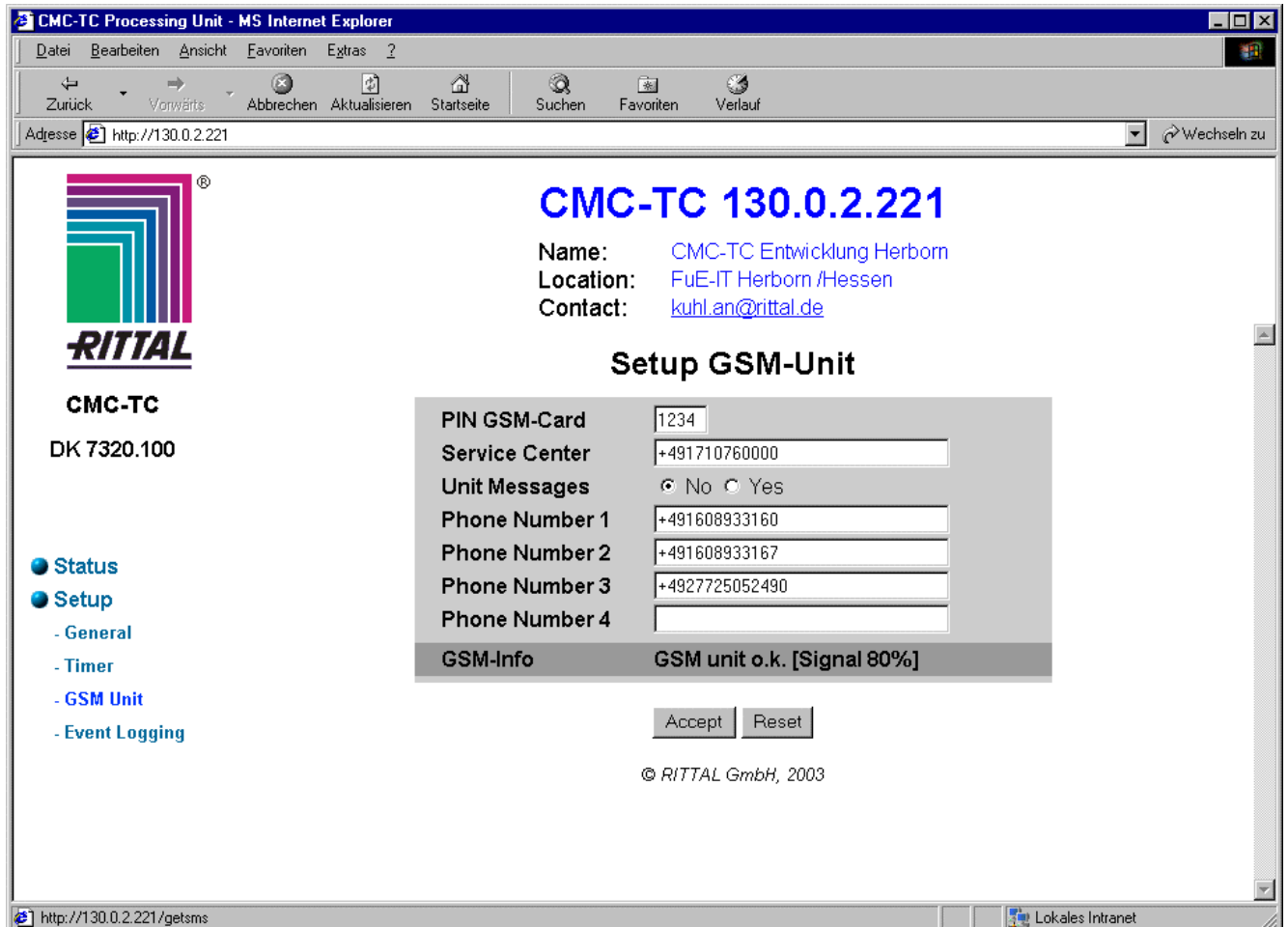
Fig. 4 GSM Unit settings via a Web browser
